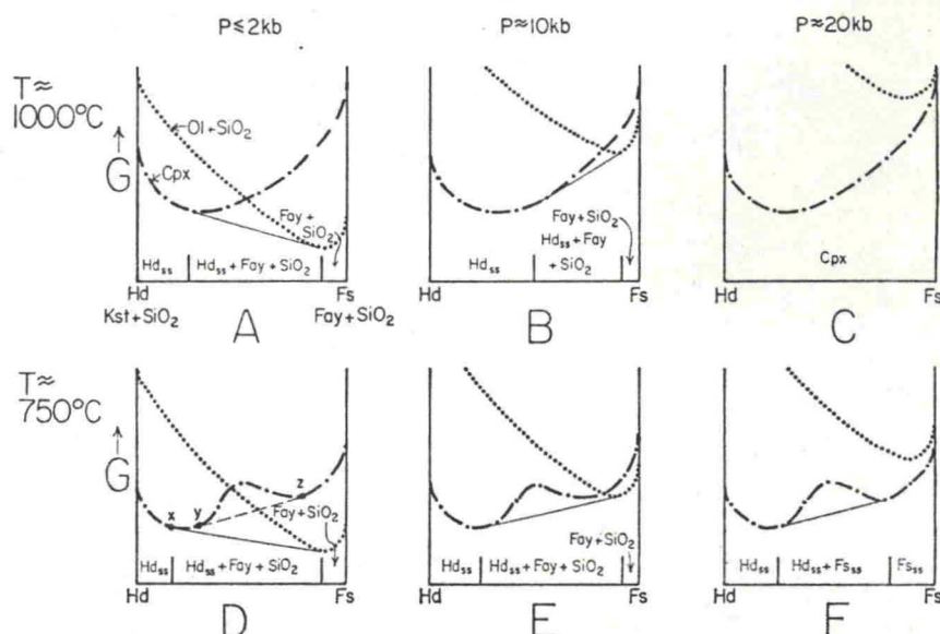
Fig. 4. Schematic free energy-composition diagrams plotted as a function of 3 pressures for temperatures of 1000°C and 750°C. Dash-dot lines: free energy for clinopyroxene solid solutions; dotted lines: free energy for equimolar olivine + \text{SiO}_2 mixtures. Polymorphism in ferrosilite is not considered. Solid tangent lines connect coexisting stable phases, and dashed tangent line (y-z in D) connects two coexisting metastable clinopyroxenes. The high temperature sections (A-C) show the effect of pressure on increasing the solubility of \text{FeSiO}_3 in \text{Ca}_{0.5}\text{Fe}_{0.5}\text{SiO}_3 ; at 20 kb there is complete solid solution along the join. At lower temperatures (D-F) a miscibility gap in the clinopyroxene series is assumed to exist. This miscibility gap is metastable at low pressures (D, E) but becomes stable at high pressures (F). From (D) it is obvious that at low pressures the metastable miscibility gap (y-z) must always be to the right of the stable curve defining the composition (x) of \text{Hd}_{ss} in equilibrium with \text{Fay} + \text{SiO}_2 . Note that it is impossible to demonstrate the existence of a metastable miscibility gap at low pressures inasmuch as the stable assemblages shown in A and D are identical.
